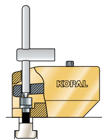
Simple and quick mounting with M 10 screw [provided]
